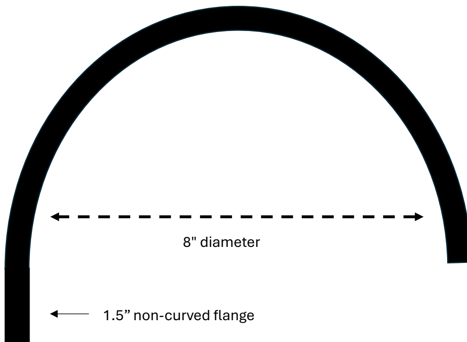
Figure 1. Cross section view of 14-inch-wide, 18-gauge galvanized sheet metal formed into a half-circle with an 8-inch diameter and a 1.5-inch unbent flange.
